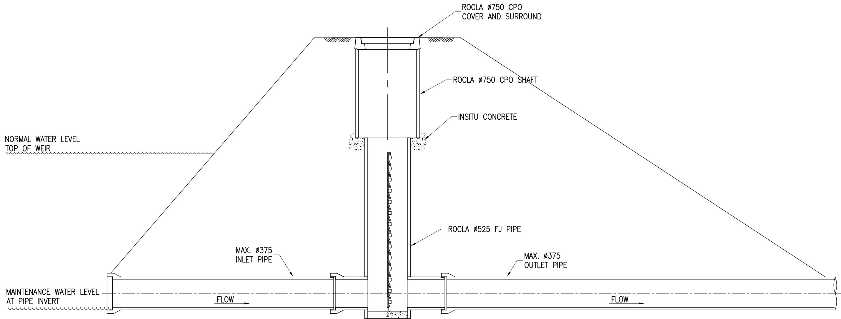
SECTION THROUGH WETLAND WALL (SCHEMATIC ONLY)
